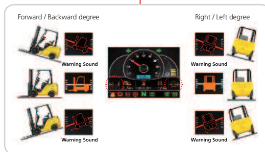
Truck Inclination Warning System
