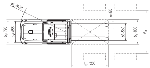
Single lift mast 2000/2500 without auxiliary lift
