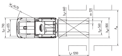
Single lift mast 2000/2500 with auxiliary lift
